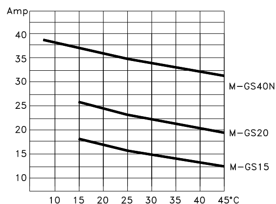
Thermal curves
